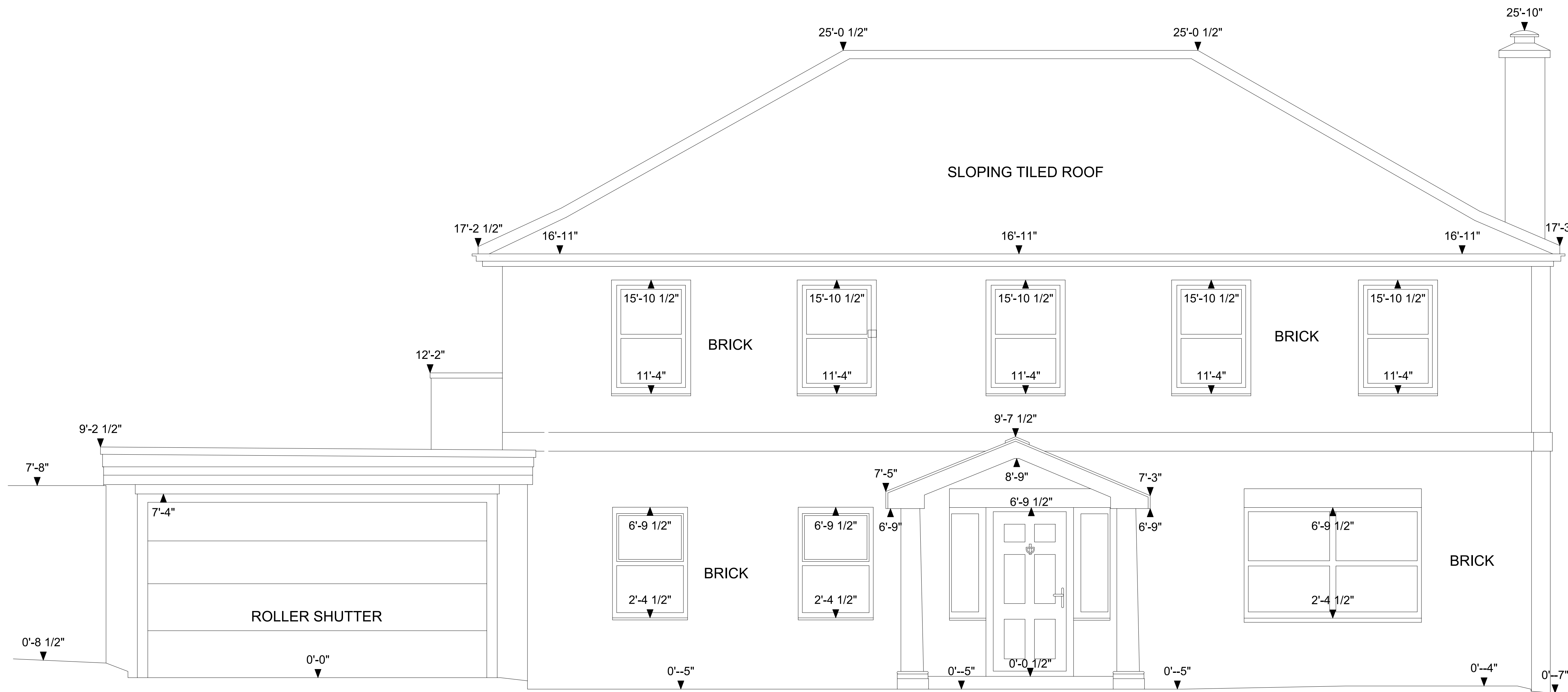
1 Elevation 1
